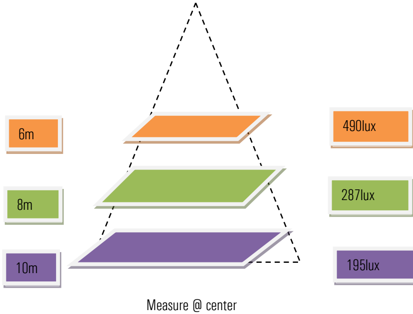
Isolux Diagram(100°)
