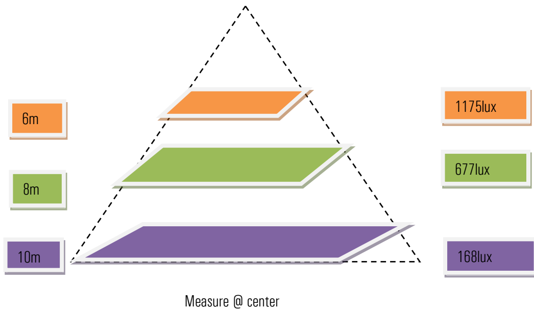
Isolux Diagram(100°)
