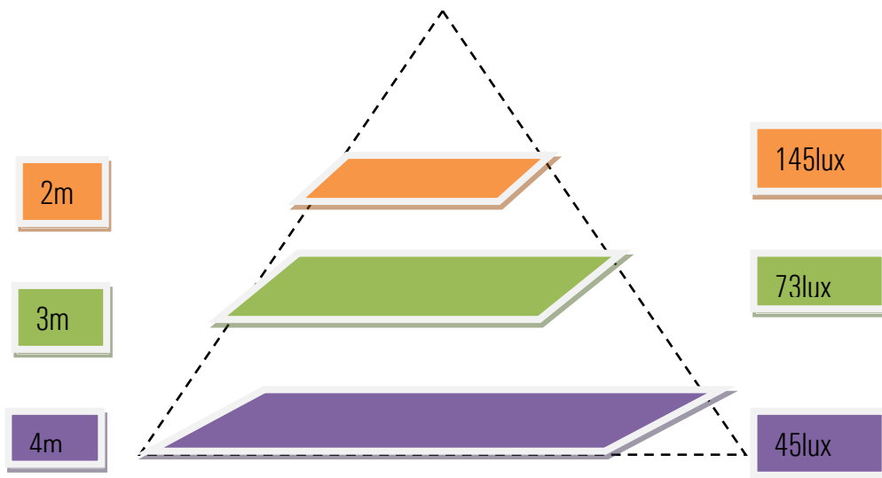
Isolux Diagram (100°)
