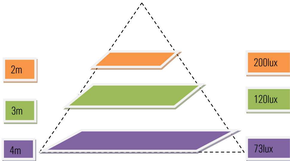
Isolux Diagram(100°)
