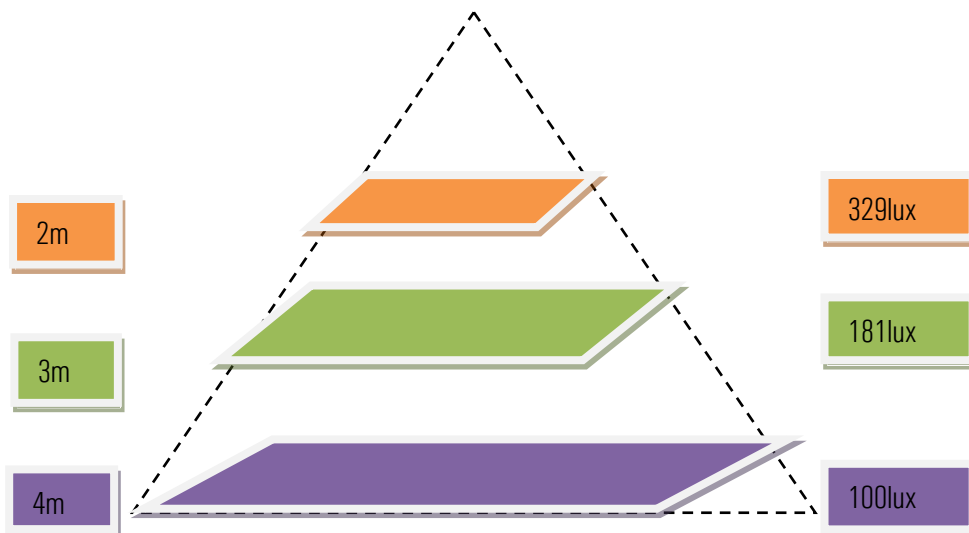
Isolux Diagram (100°)
